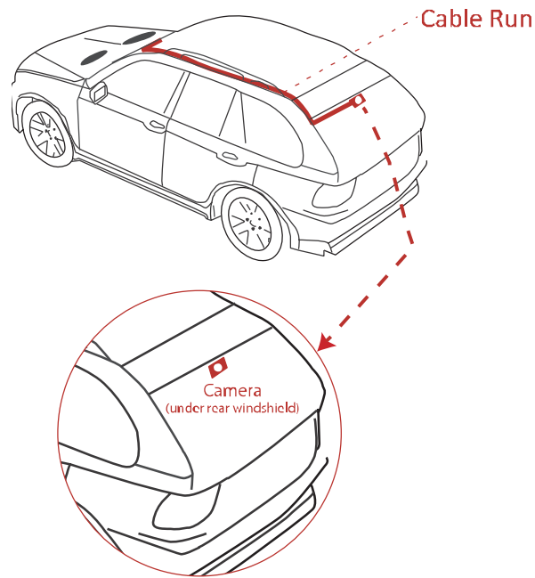
Figure 7, Rear Camera Interior Cable Run
