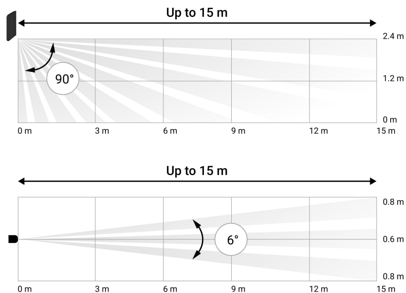
Horizontal and vertical detector's angles of view
